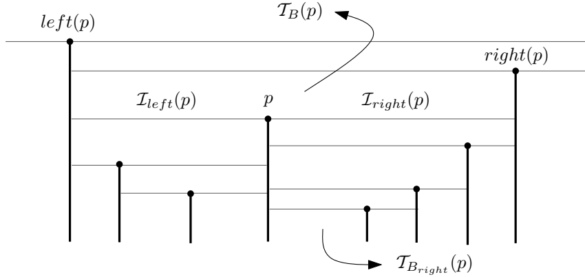
Figure 3: Details of \mathcal{D}(p_r) .
