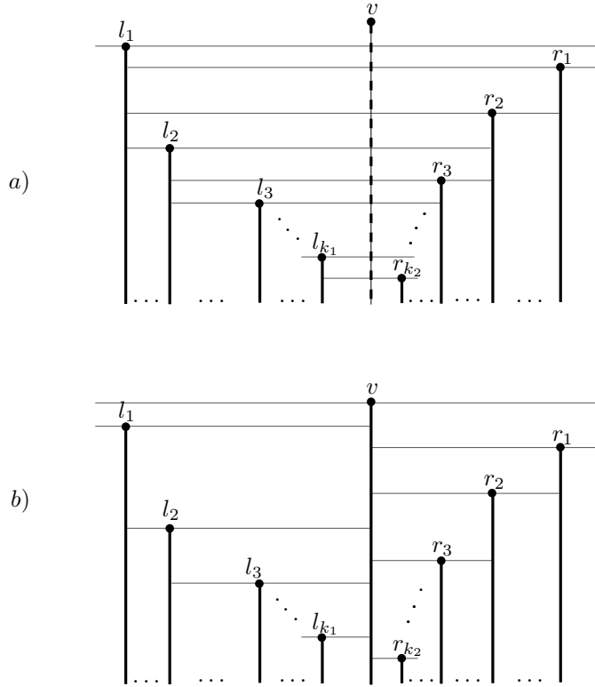
Figure 7: Inserting a red point v in \mathcal{D}(p_r) . a) Before insertion, b) After insertion.
