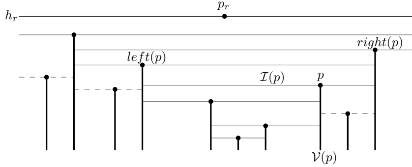
Figure 2: \mathcal{D}(p_r) . Candidate points are those whose \mathcal{I}(p) is drawn with a continuous line.
