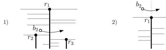
Figure 5: Two cases of vertical flip between a red point r_1 and a blue point b_2 .
