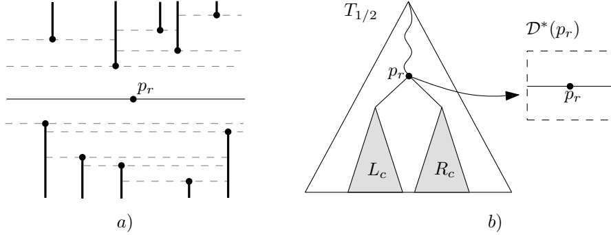
Figure 8: a) \mathcal{D}^*(p_r) , b) The Two-Level Data Structure for the approximation.
