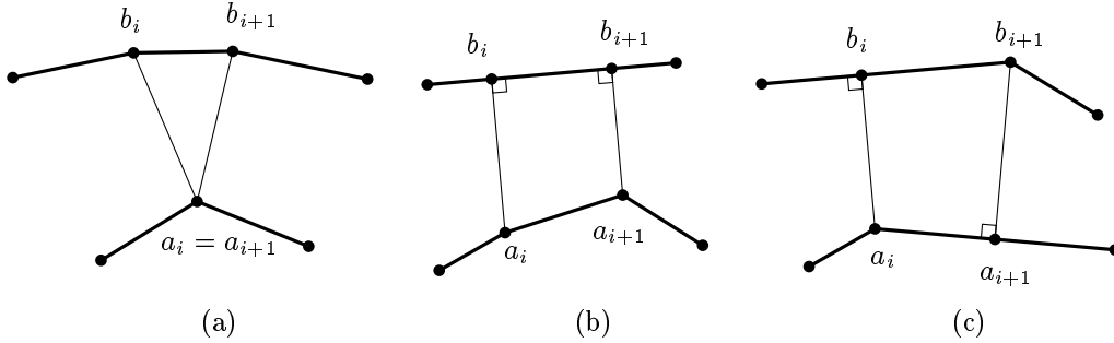
Fig. 6. Transition property for (a_i, b_i) and (a_{i+1}, b_{i+1}) .
