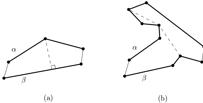
Fig. 3. Two cases of the minimum width morphing.
