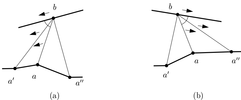
Fig. 4. Changing critical matches (a) a'b and ab , and (b) ab and a''b .
