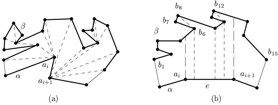
Fig. 7. (a) Shortest path tree T_{a_{i+1}} . (b) Vertices b_6, b_7, \dots, b_{12} form shortest paths to e .
