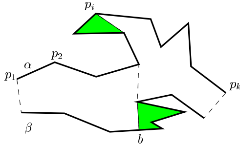
Fig. 8. Pockets are shaded.
