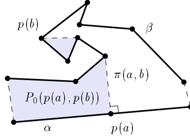
Fig. 5. Morph F_{a,b} in shaded polygon.
