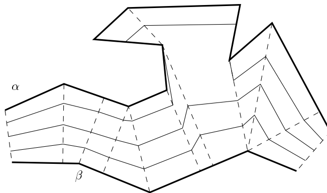
Fig. 1. Morphing between two polylines \alpha and \beta .
