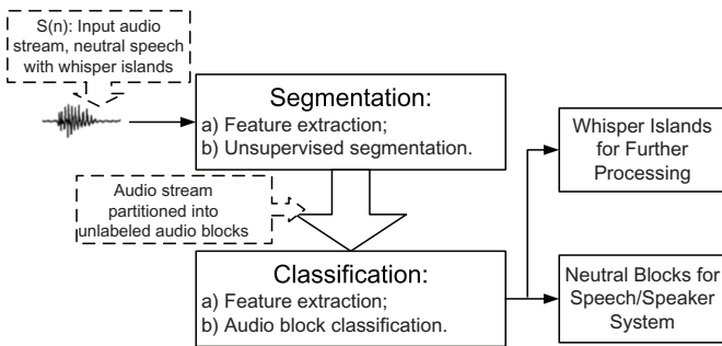
Fig. 1: High Level Flow Diagram of Whisper-Island Detection
