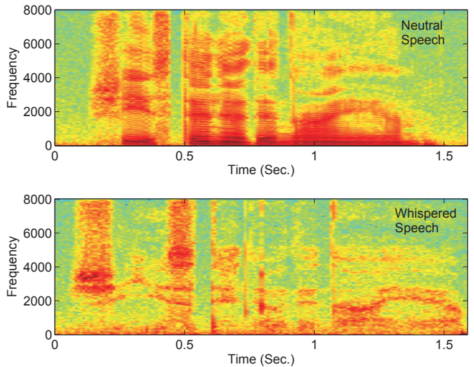
Fig. 3: Spectrograms of Neutral Speech Signal and Whispered Speech Signal
