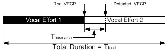
Fig. 13: Illustration of how boundary mismatch(in msec) is converted to overall boundary mismatch rate(in %): Mismatch\% = \frac{T_{mismatch}}{T_{total}} \times 100\%
