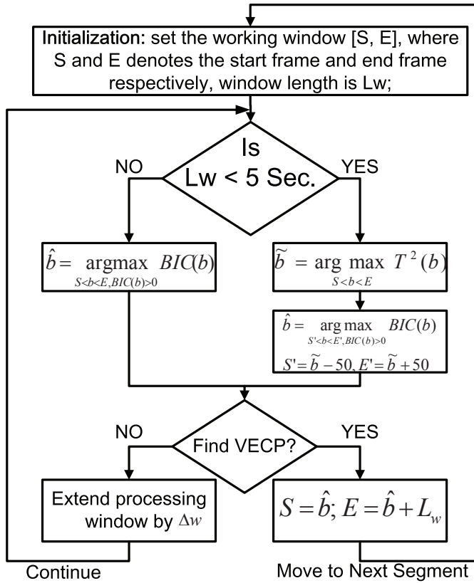
Fig. 14: Segmentation based on BIC/ T^2 -BIC processing algorithm for VECP detection
