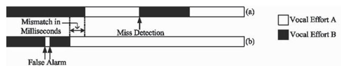
Fig. 12: Three Types of Segmentation Error for Whisper Islands in Audio Streams.
