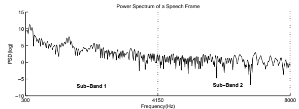
Fig. 11: The Two Sub-Band over Frequency Domain for Whisper Analysis
