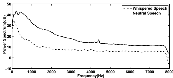
Fig. 9: Power Spectrum Amplitude for Whispered Speech and Neutral Speech
