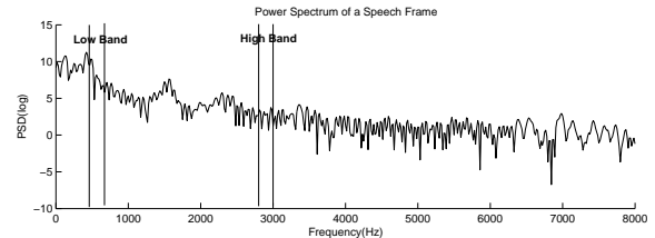
Fig. 10: Entropy Ratio between High Frequency Band and Low Frequency Band
