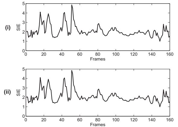
Fig. 8: SIE sequence of the speech signals shown in Fig. 7
