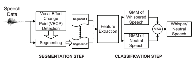
Fig. 6: Flow Diagram of Whisper-Island Detection.
