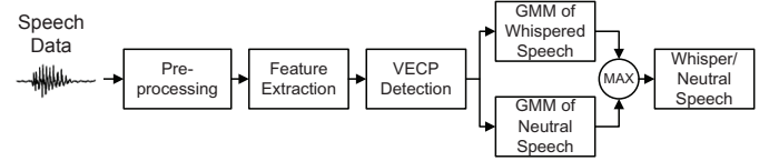
Fig. 16: The Flow Diagram of Entire System: (i) segmentation, followed by (ii) whisper/neutral classification.
