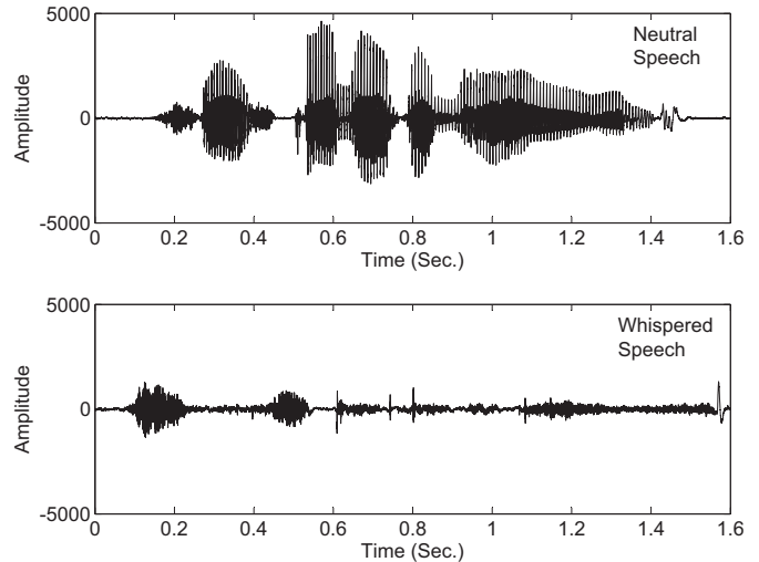
Fig. 2: Waveforms of Neutral Speech and Whispered Speech Signals for the Phrase “She is thinner than I am”.
