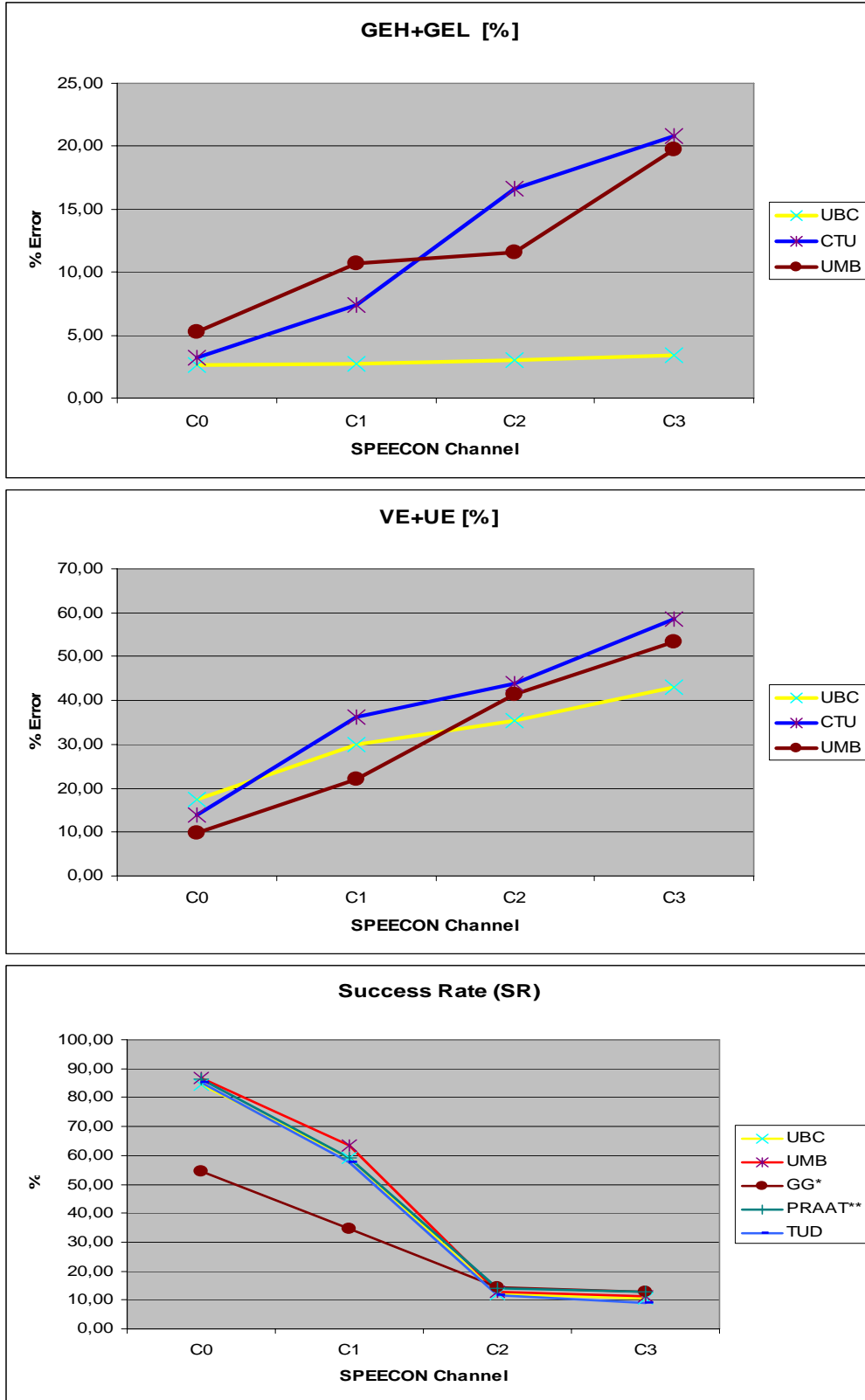
Fig.1 Error rates of pitch detection (PDA) and pitch marking (PMA) algorithms
