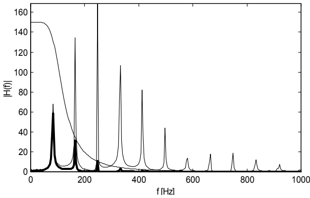
Figure 3: Spectral shaping by low-pass IIR.
