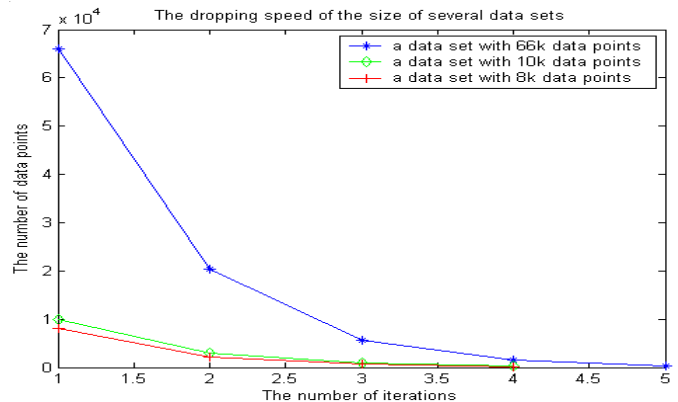
Figure 4. The dropping speed of the size of several testing data sets when applying GraphZip
