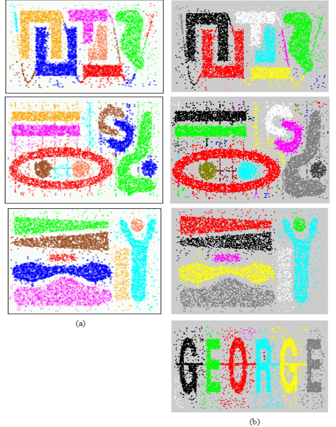
Figure 6. The clustering results of (a) CHAMELEON; (b) GraphZip
