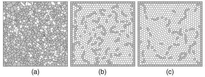
Fig. 7. (a) The Voronoi diagram of 1,000 initial sites in the 2D domain of [-1, 1] \times [-1, 1] , and CVT results generated by the L-BFGS algorithm using (b) GPU, and (c) CPU. (Unshaded cells are hexagons.)
