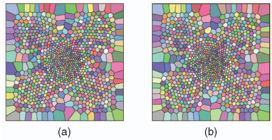
Fig. 9. CVT results of 1,000 initial sites generated by the L-BFGS algorithm in the 2D domain of [-1, 1] \times [-1, 1] with the density function \rho(x) = e^{-20x^2 - 20y^2} + 0.05 \sin^2(\pi x) \sin^2(\pi y) using (a) GPU and (b) CPU.
